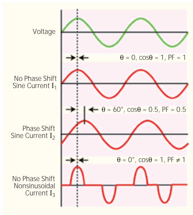
Figure 2. Current Waveforms for Different Power Factors
