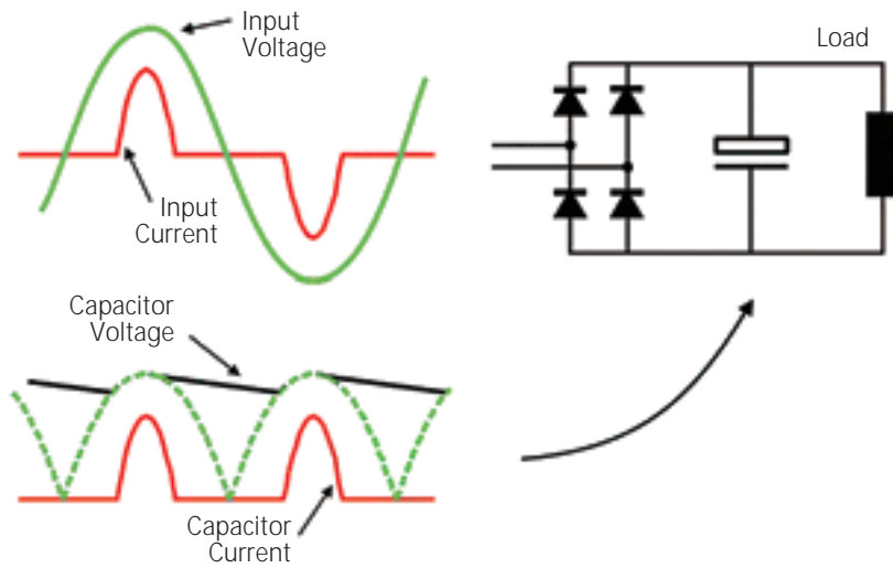
Figure 1. Voltage and Current Waveforms of a Full-Wave Rectifier
